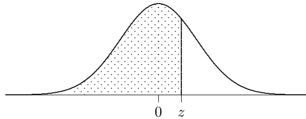
The standard normal distribution
